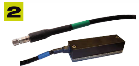
2 Load sensors to read suspension pressure or, depending on the application, axle-mounted sensors
